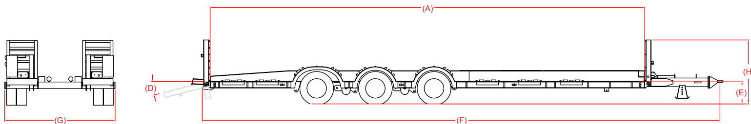
Forestry trailer
